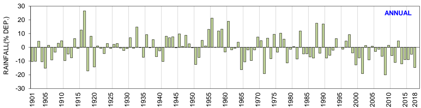
Fig. 2: Time Series of All India Annual Rainfall percentage Departure 901-2018)
