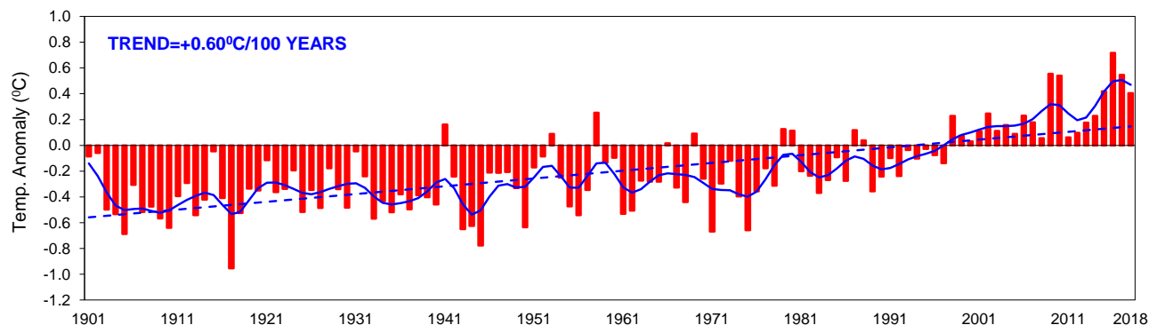
Fig.1: Annual mean land surface air temperatures anomalies averaged over India for the period 1901-2018. The anomalies were computed with respect to base period of 1981-2010. The dotted line indicates the linear trend in the time series. The solid blue curve represents the sub-decadal time scale variation smoothed with a binomial filter.
